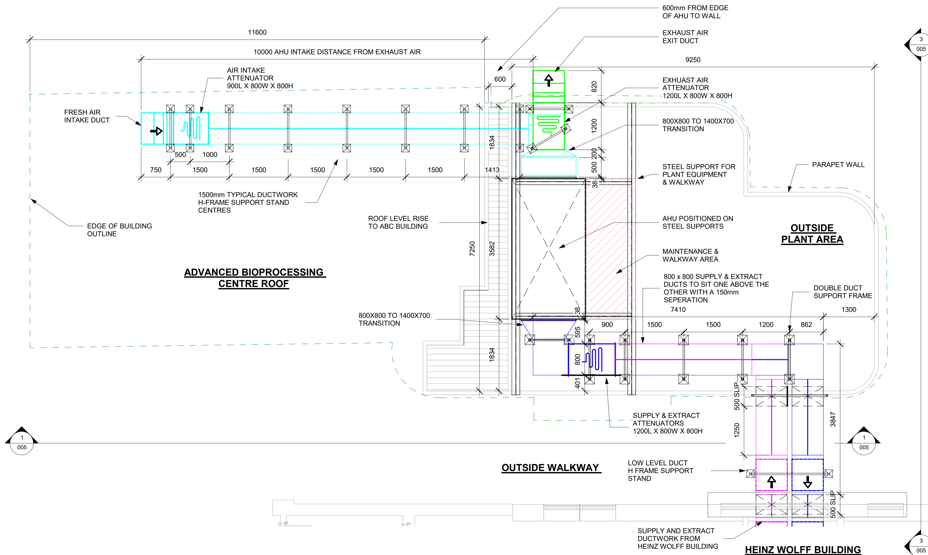
2 Outside Plant Area - Plan 1 : 50
